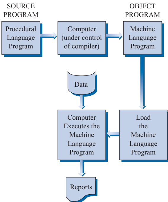
FIGURE 2.10 Compiling and Running a Procedural Language Program
